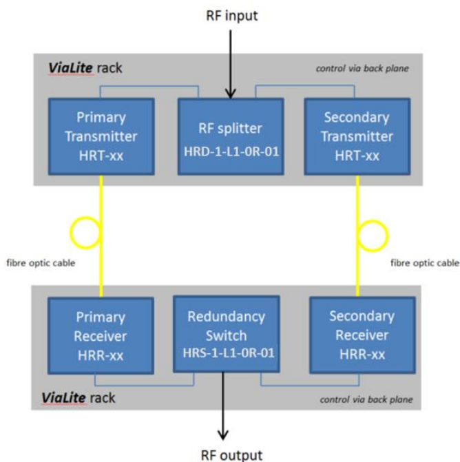
Typical 1:1 redundancy configuration
