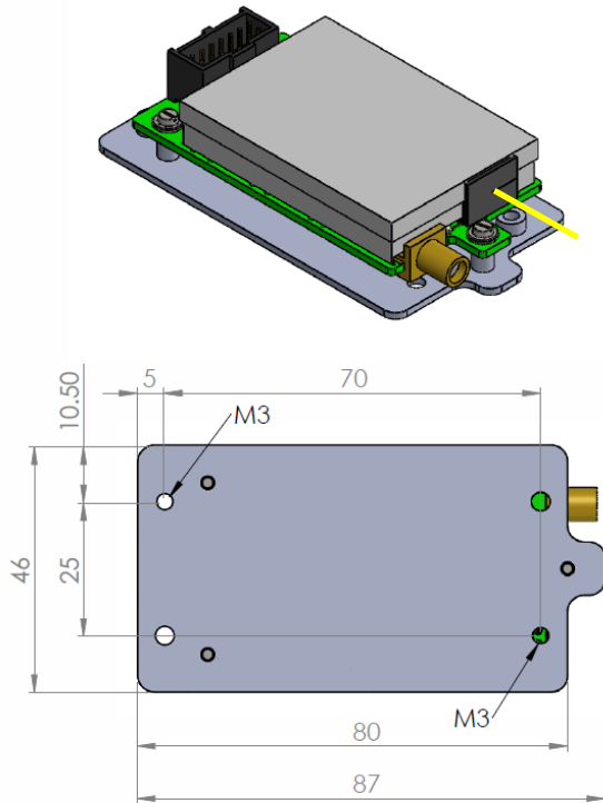
C type module with an adaptor plate, in mm View looking from bottom of the module
