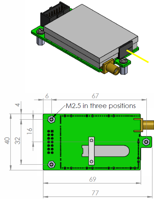
B type module with stand-off, in mm View looking from bottom of the module
